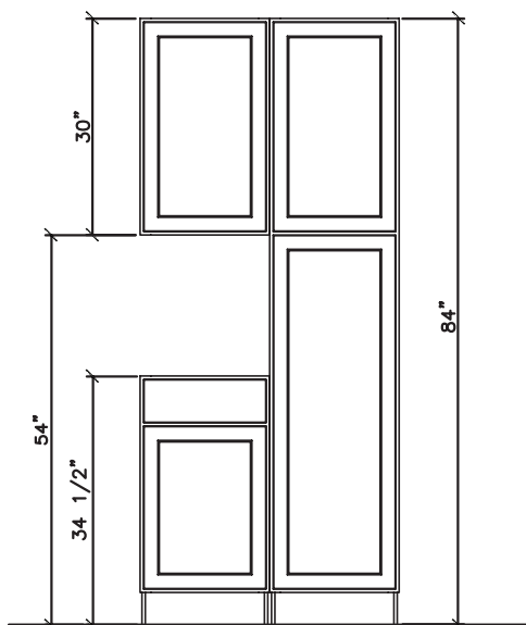
84" tall cabinet with 30" high wall cabinet
